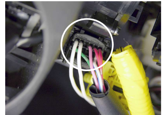
Insert the Black and White/Purple wire in to the connector in pin 7 and 8. Placement is unimportant.
