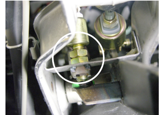
The pedal stop is measured and replaced by the enclosed clutch switch. The clutch switch must be placed on the same level as the pedal stop.
