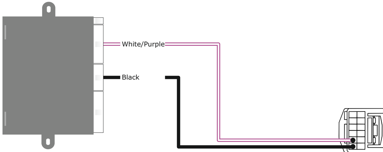
Connector below steering wheel (Viewed from wire side)
